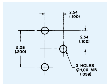
Plan T
