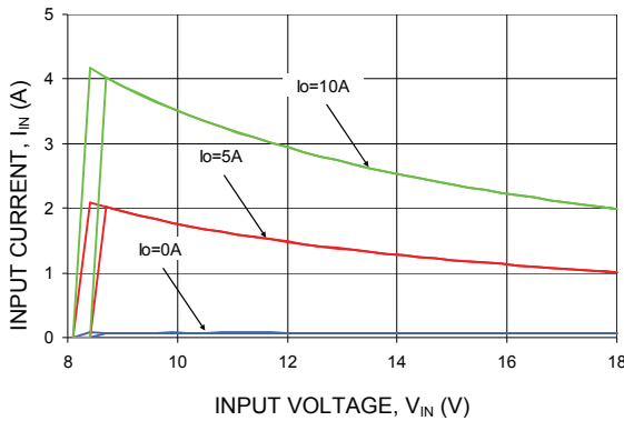
Figure 7. Input voltage vs. Input Current (V out = 3.3Vdc).
