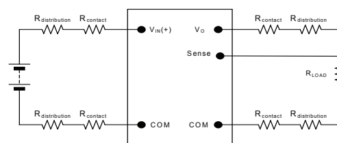
Figure 30. Remote sense circuit configuration
