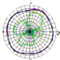
Azimuth Plane, 1910 MHz
