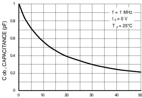
Figure 14. Output Capacitance
