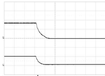
Shut-down enabled by disconnecting V_1 at: T_{ref} = +25^{\circ}C, V_1 = 53 V, I_o = 20 A resistive load.
