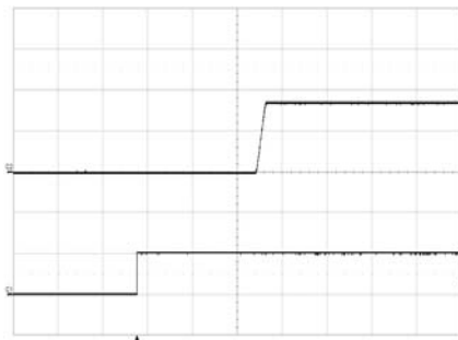
Start-up enabled by connecting V_1 at: T_{ref} = +25^{\circ}C, V_1 = 53 V, I_o = 20 A resistive load.
