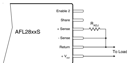
Figure V. Connection for V_{OUT} Adjustment
