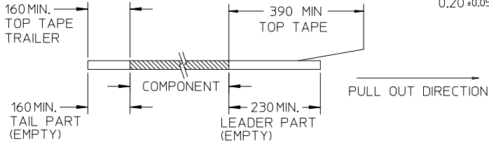
DETAIL 1
