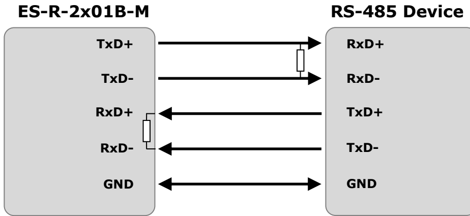
Figure 7 RS-485 Full Duplex Wiring
