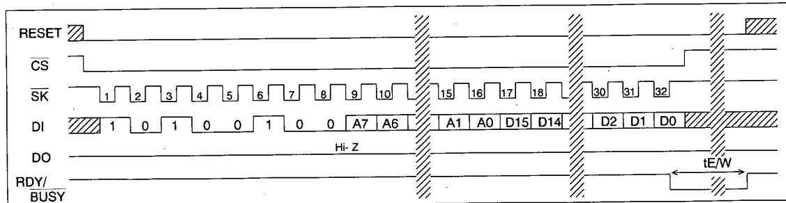
WRITE (AK6440A)
