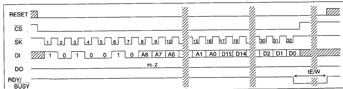
WRITE (AK6480A)
