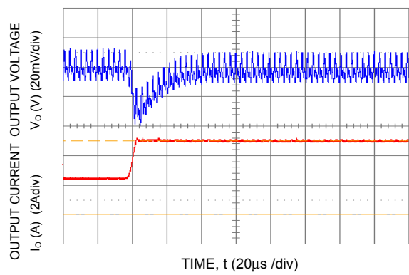
Figure 4. Transient Response to Dynamic Load Change from 50% to 100% at 28Vin, C ext - 10uF ceramic + 330uF polymer, C Tune =10nF & R Tune =150Ω
