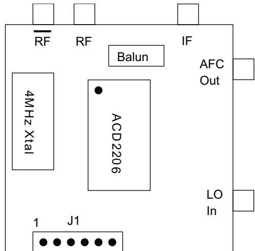
Figure 14: Evaluation Fixture
