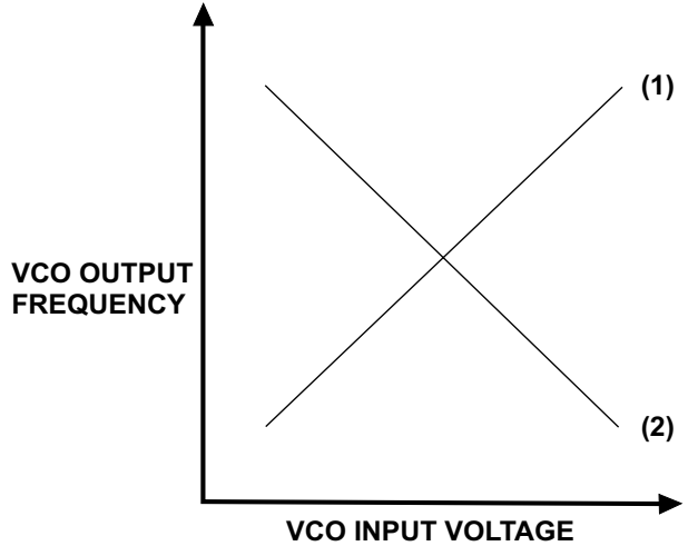
Figure 10: VCO Characteristics
