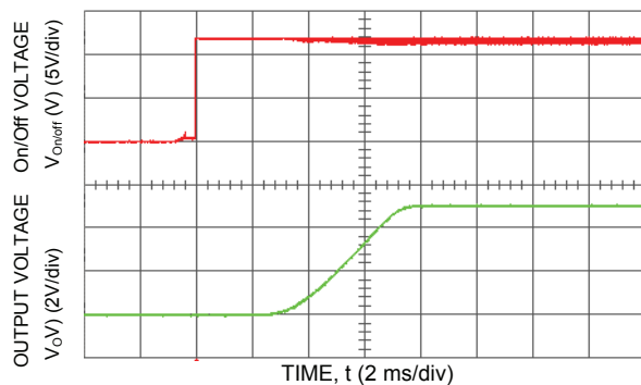
Figure 15. Typical Start-Up Using Remote On/Off with Low-ESR external capacitors (7x150µF Polymer) ( V_{in} = 12\text{ Vdc} , V_o = 5.0\text{ Vdc} , I_o = 16\text{ A} , C_o = 1050\text{ }\mu\text{F} ).
