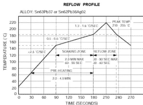
Figure 35. Reflow Profile.
