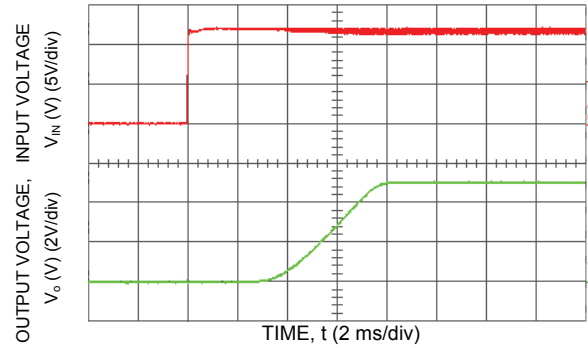
Figure 16. Typical Start-Up with application of V_{in} with low-ESR polymer capacitors at the output (7x150 \mu\text{F} ) ( V_{in} = 12\text{ Vdc} , V_o = 5.0\text{ Vdc} , I_o = 16\text{ A} , C_o = 1050\text{ }\mu\text{F} ).
