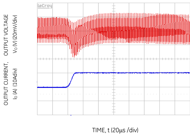
Figure 10. Transient Response to Dynamic Load Change from 50% to 100% at 12V in , C_{out} = 1 \times 47 \mu F + 5 \times 330 \mu F , C_{Tune} = 10nF & R_{Tune} = 178 \text{ ohms}
