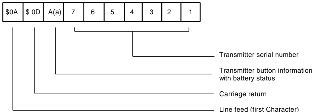
Valid Output from SD1 pin
