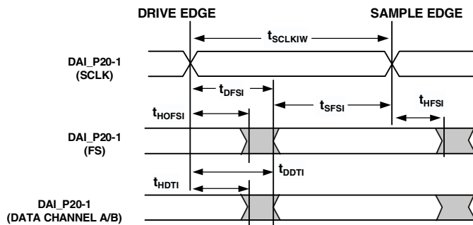
Figure 31. SPDIF Receiver Internal Digital PLL Mode Timing
