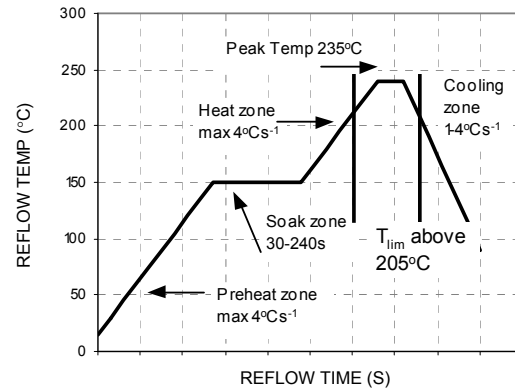
Figure 35. Reflow Profile for Tin/Lead (Sn/Pb) process
