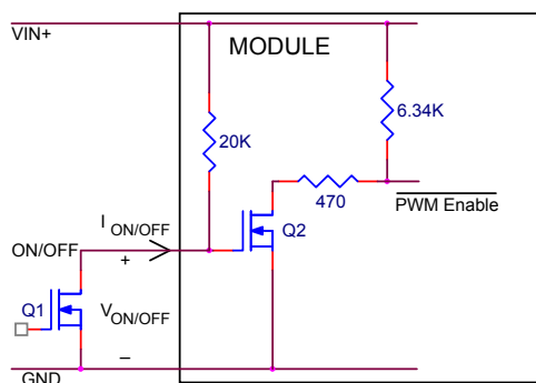
Figure 38. Circuit configuration for using positive On/Off logic.
