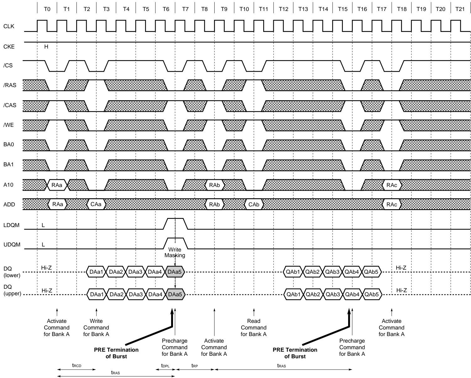
13.27 PRE (Precharge) Termination of Burst (1/2) (Burst Length = 8, /CAS Latency = 2)
