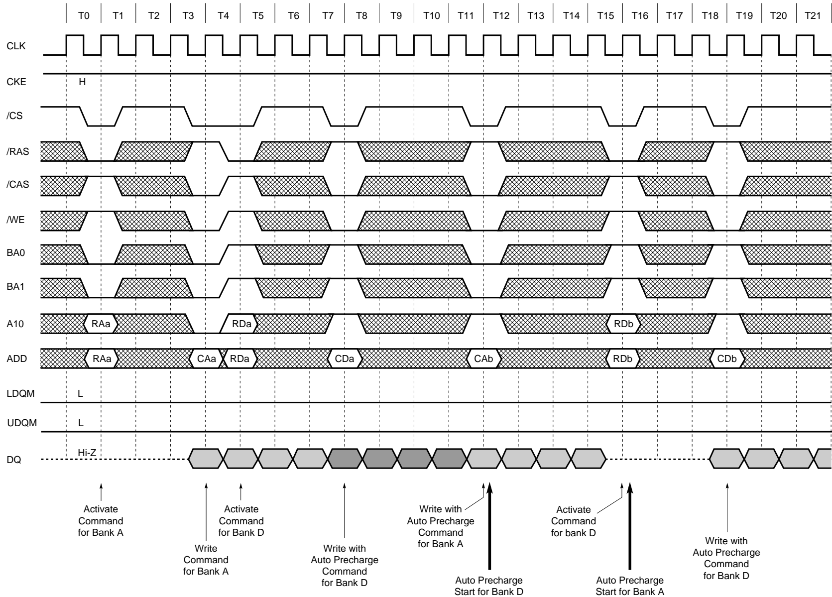
Auto Precharge after Write Burst (2/2) (Burst Length = 4, /CAS Latency = 3)
