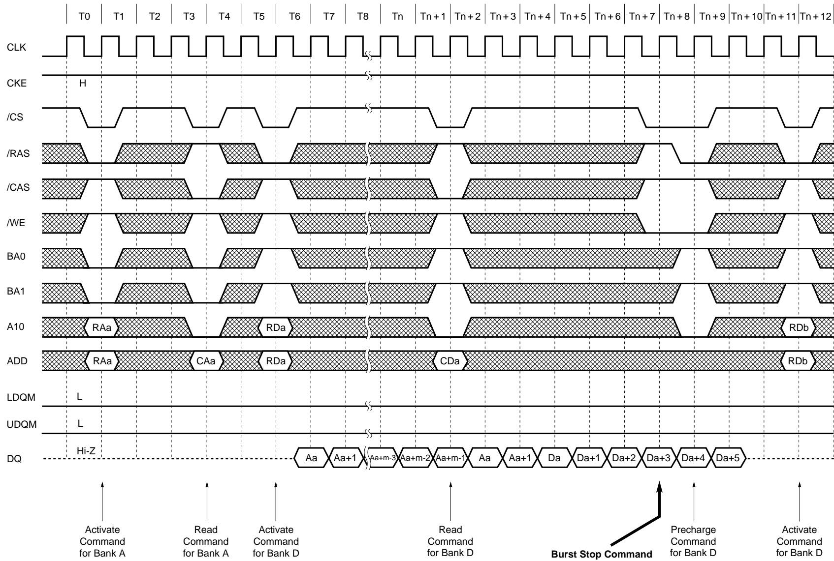
Full Page Read Cycle (2/2) (/CAS latency = 3)
