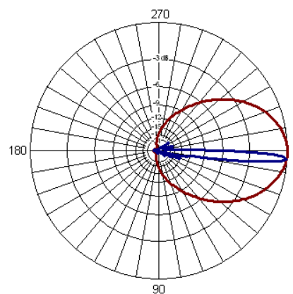
4 DEGREE DOWN TILT PLOT
