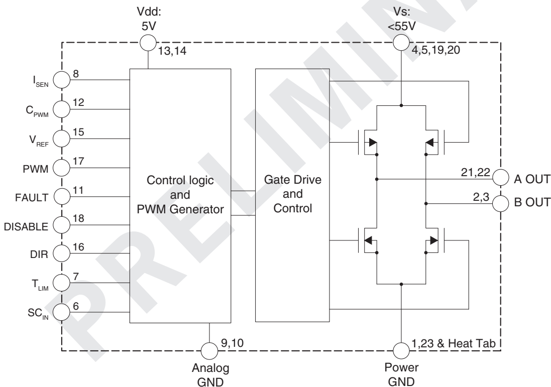
FIGURE 1. BLOCK DIAGRAM
