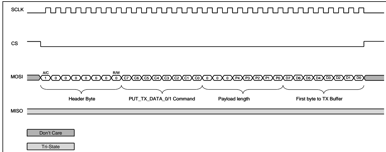
Figure 15. PUT_TX_DATA_0/1 Command
