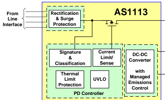
Figure 15 – Top-Level Block Diagram of the AS1113
