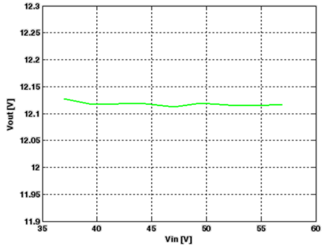
Figure 12 - DCDC Line Regulation @ I_{OUT}=0.25A
