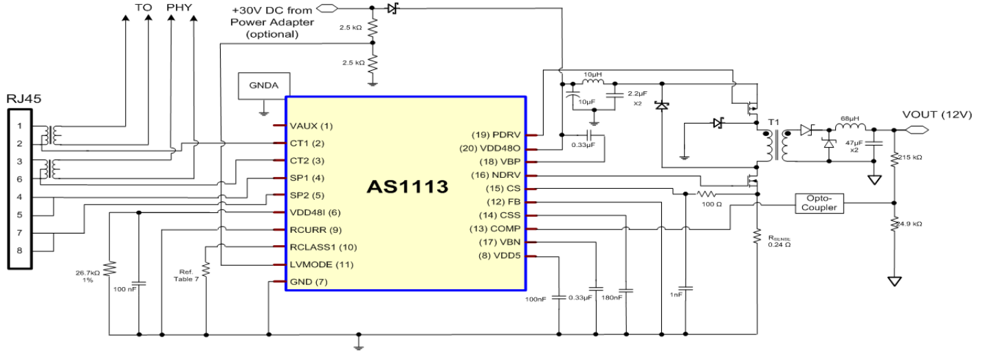
Figure 20 – 10/100M with Forward DC-DC converter
