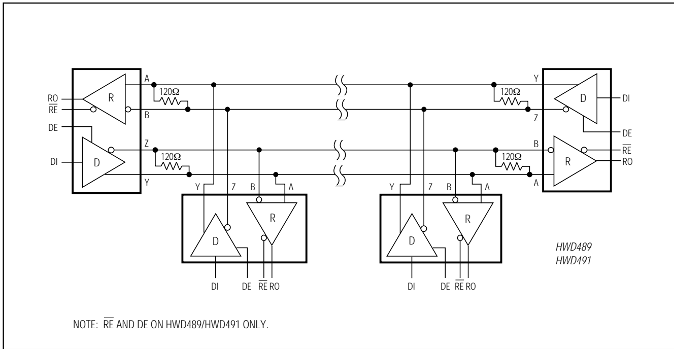
Figure 22. HWD488-HWD491 Full-Duplex RS-485 Network
