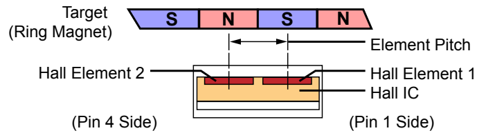
Figure 1: Relative motion of the target is detected by the dual Hall elements mounted on the Hall IC.
