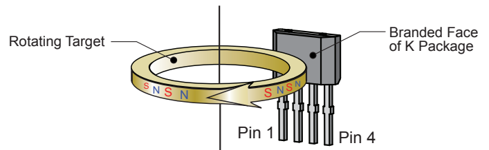
Figure 2: This left-to-right (pin 1 to pin 4) direction of target rotation results in a high output signal when a target north pole is nearest the face of the device (see figure 3). A right-to-left (pin 4 to pin 1) rotation inverts the output signal polarity.
