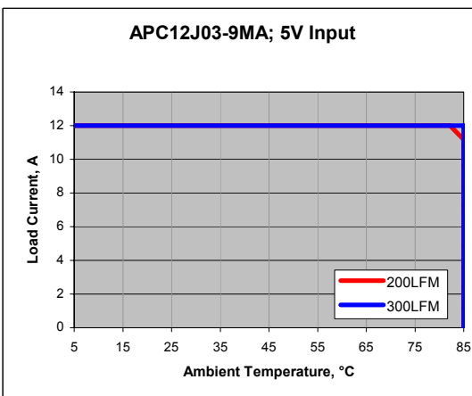
Figure 24. J03 – Load current vs. ambient temp.
