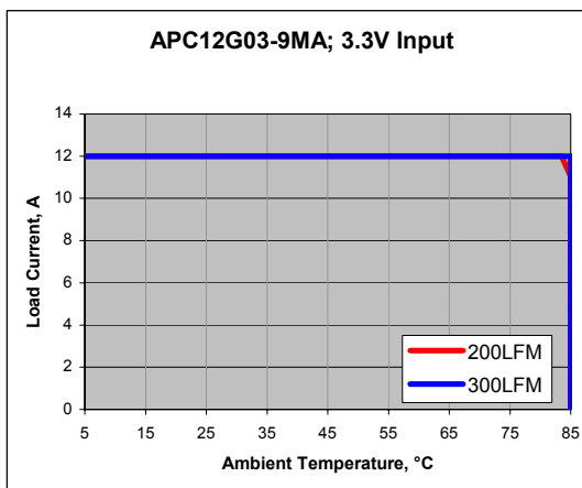
Figure 20. G03 – Load current vs. ambient temp.
