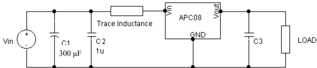
Figure 2a. Typical Application Circuit.
