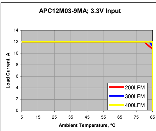
Figure 22. M03 – Load current vs. ambient temp.
