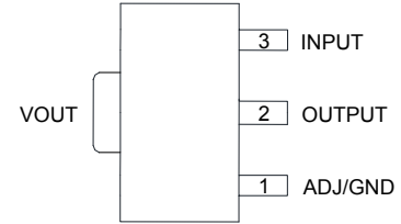
(SOT89-3L Option 2/ R Package)
