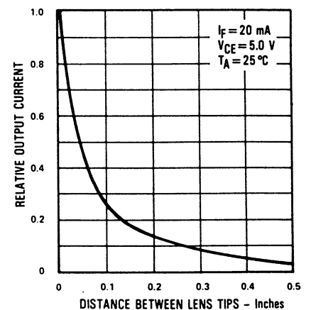
Coupling Characteristics of OP165W and OP505W
