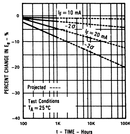
Percent Changes in Power Output vs Time
