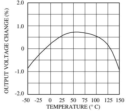
Temperature Stability
