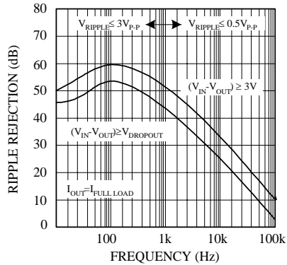
Ripple Rejection
