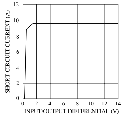
Short-Circuit Current
