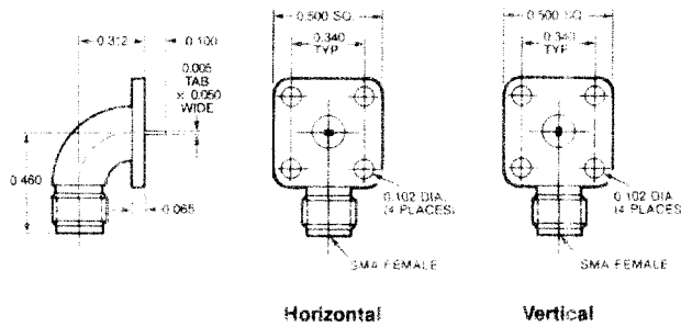
Radius Right Angle Flange Mount Female
