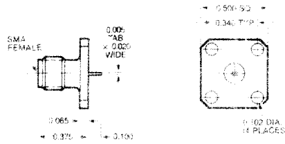
Flange Mount Female .020 Wide Tab
