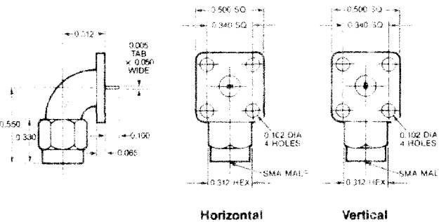
Radius Right Angle Flange Mount Male
