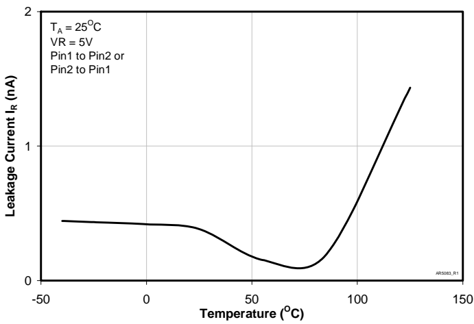
Typical Leakage Current v Temperature
