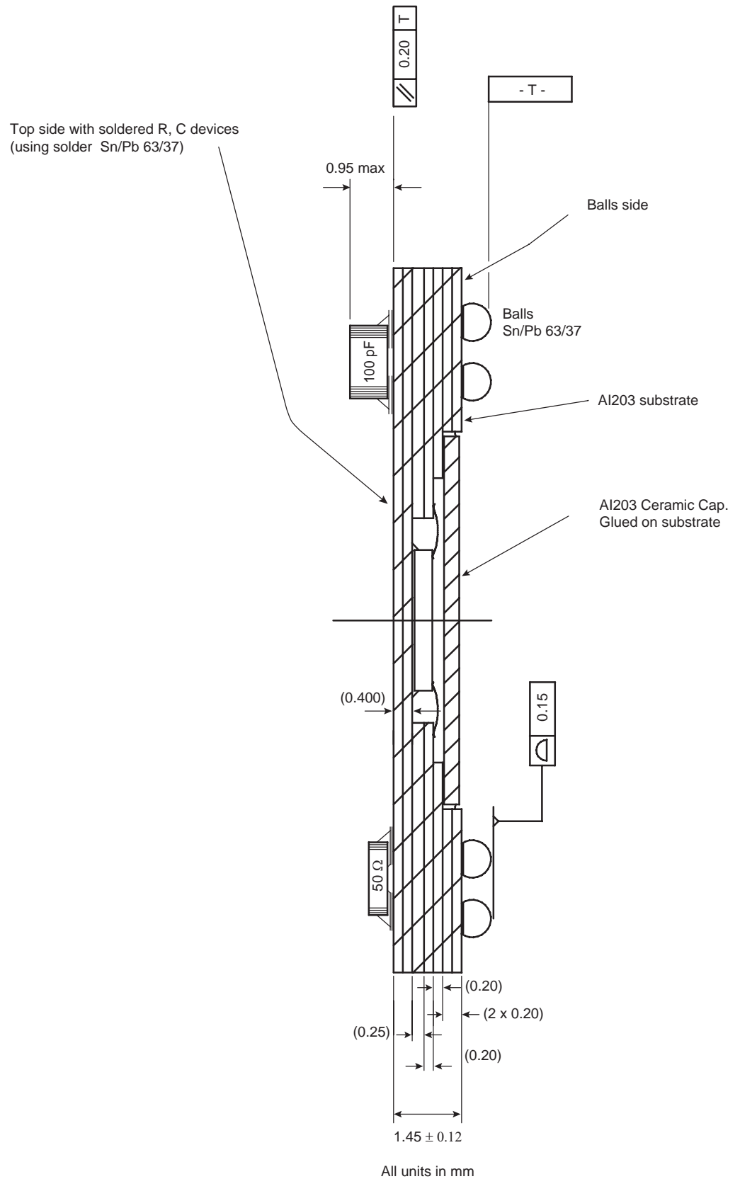
Figure 50. Cross Section
