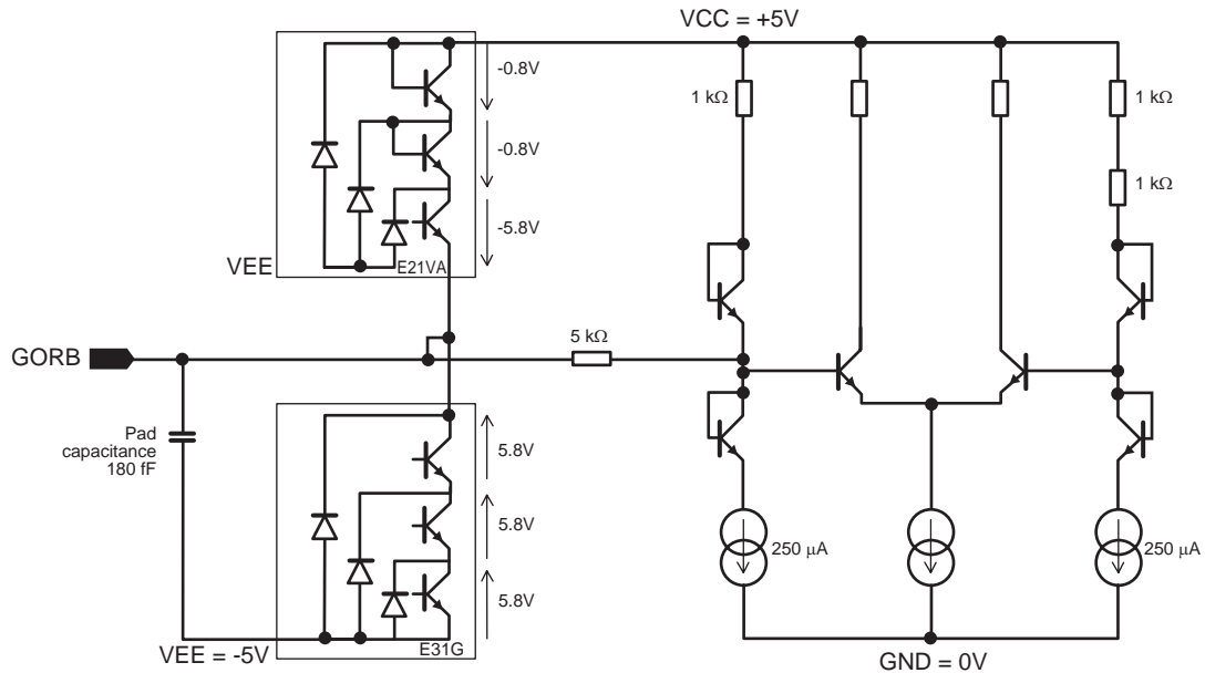
Figure 45. GORB Equivalent Input Schematic and ESD Protections
