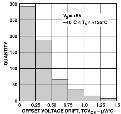
FIGURE 4. INPUT OFFSET VOLTAGE DRIFT DISTRIBUTION
