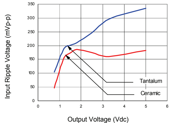
Figure 26. Input ripple voltage for various output with 6 \times 47 \mu F tantalum capacitors and with 6 \times 22 \mu F ceramic capacitors at the input (full load).
