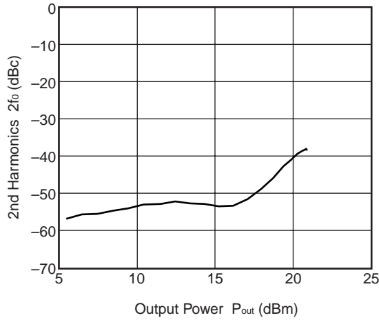
2ND HARMONICS vs. OUTPUT POWER
