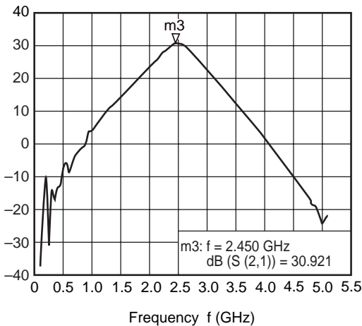
S 21 -FREQUENCY
