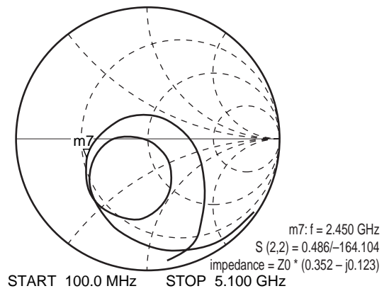
S 22 -FREQUENCY
