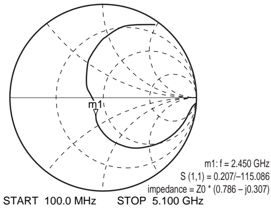
S 11 -FREQUENCY
