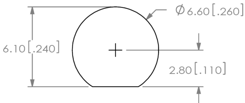
Figure 2 Recommend Cutout
