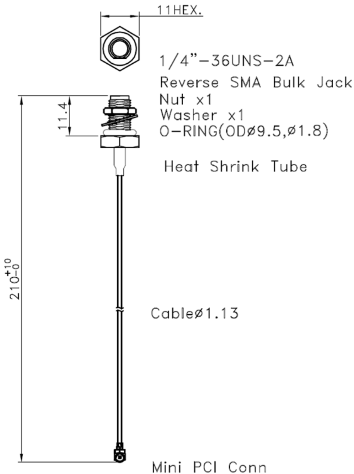
Figure 1 Physical Dimensions
