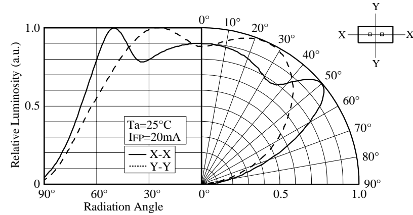
■ Directivity
