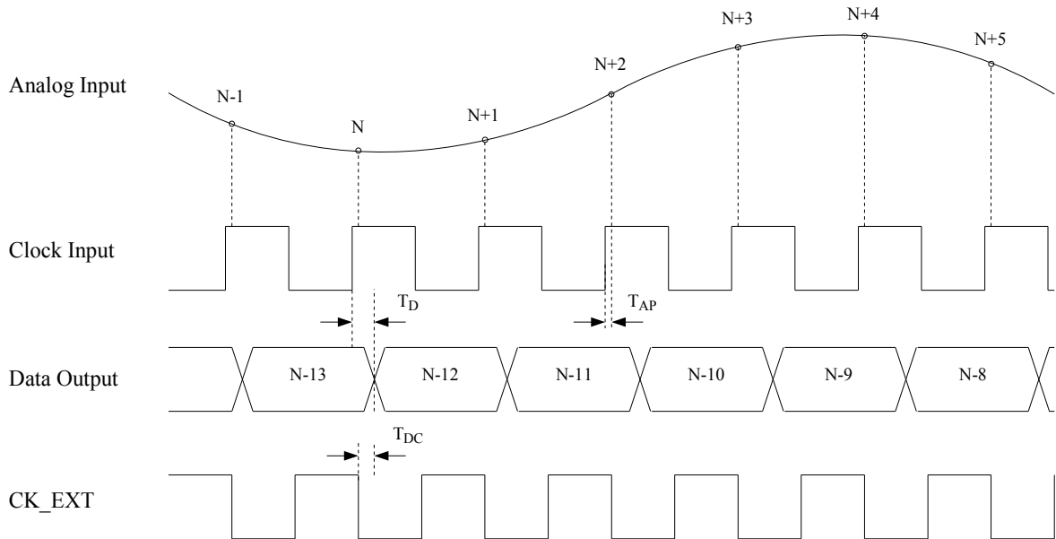
Figure 2: Timing Diagram
