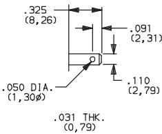
05 .110" QUICK CONNECT
