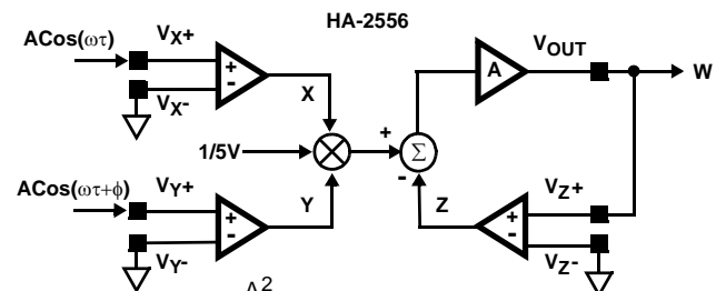
FIGURE 8. PHASE DETECTION
