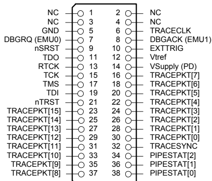
FIGURE 36 The pinout of the ETM38 connector when used with ARM targets.
