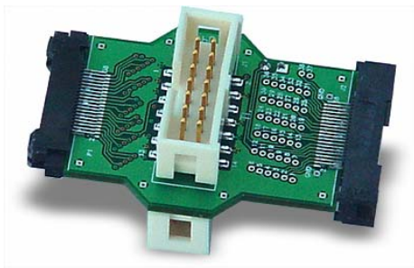
FIGURE 37 The JTAG-ETM splitter probe.
