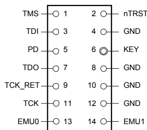
FIGURE 27 The TI14 pinout of the ADA-ISO-TI14-E probe. Top view.
