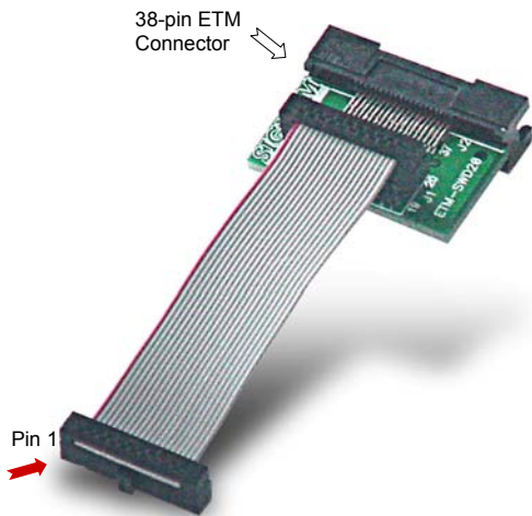
FIGURE 40 The ADA-ETM-SWD20 probe for Cortex boards with ETM trace.
