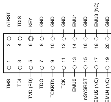
FIGURE 31 The cTI20 pinout of the ADA-JET-CTI20 probe. Top view.
