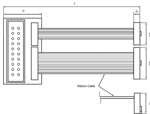
FIGURE 16 The dimensions of the ADA-ARM20-SWD probe. C = 23.6 mm (0.93 in), D = 3.11 mm (0.122 in), H = 5.1 mm (0.2 in), L = 69.3 mm (2.73 in), W = 15.73 mm (0.62 in), W1 = 10.5 mm (0.41 in), W2 = 16.9 mm (0.67).
