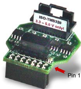
FIGURE 21 The JTAGjet TMS320 ADA-ISO-TI14 isolation probe.
