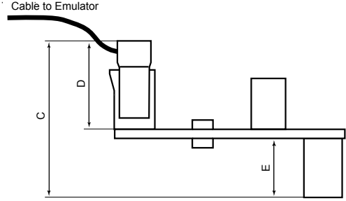
FIGURE 29 The ADA-ISO-TI14-E probe. Side view. C = 20.5 mm (.81 in.), D = 14.2 mm (0.56 in.), E = 8.5 mm (0.33 in.).
