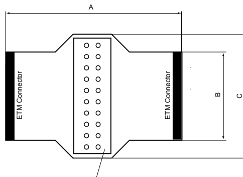
FIGURE 38 The dimensions of the JTAG-ETM splitter board. A = 52.0 mm (2.05 in), B = 25.4 mm (1 in), C = 33.9 mm (1.34 in).
