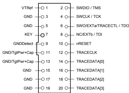
FIGURE 42 The Cortex20 pinout of the Cortex side of the ADA-ETM-SWD20 probe. Top view.
