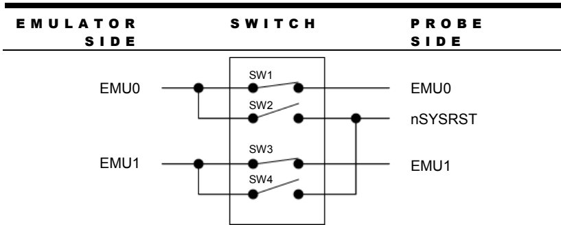
FIGURE 34 The DIP switches SW1-4 on the CTI20 probe in default setting positions.
