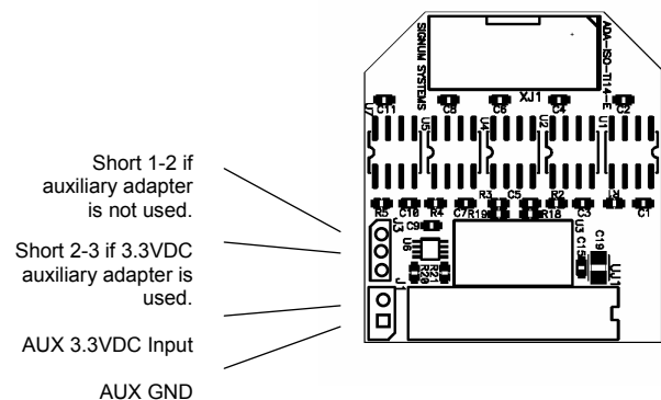
FIGURE 25 An early version of the ADA-ISO-TI14-E with jumper-controlled auxiliary power input.
