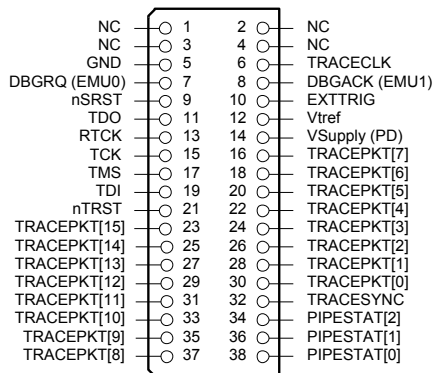
FIGURE 43 The ETM32 pinout of the ETM side of the ADA-ETM-SWD20 probe. Top view.
