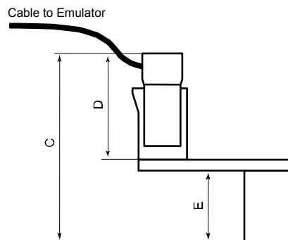
FIGURE 33 Dimensions of the 20-pin CTI20 probe. Side view. C = 23.0 mm (.91 in.), D = 12.5 mm (0.49 in.), E = 6.4 mm (0.25 in.).
