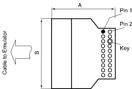
FIGURE 32 Dimensions of the 20-pin CTI20 probe. Top view. A = 27.0 mm (1.06 in.) B = 17.8 mm (0.70 in.).
