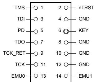
FIGURE 18 The TI14 pinout of the 14-pin JTAGjet probe for OMAP and TMS320 DSP. On the right, a top view of a matching probe layout for a target board.
