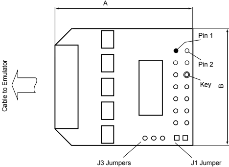
FIGURE 28 The dimensions of the 20-pin ADA-ISO-TI14-E probe. Top view. A = 32.4 mm (1.28 in), B = 28.5 mm (1.12 in).
