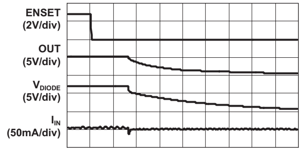
Turn-Off
