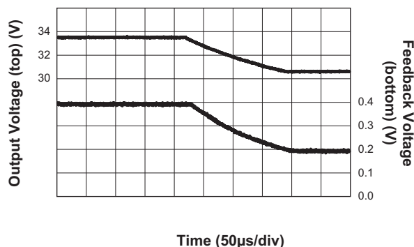
Transition of LED Current (10 White LEDs; SEL = Low; I_{LED} = 13\text{mA} to 6\text{mA} )
