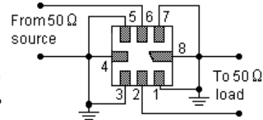
Test Circuit
