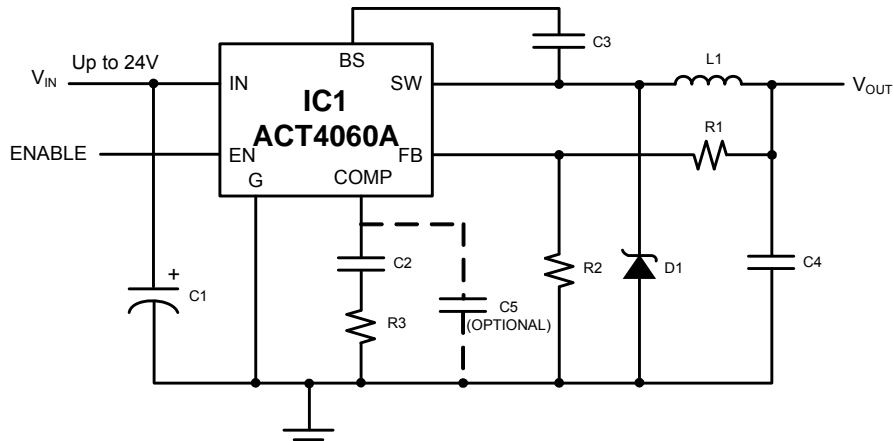
Figure 3: ACT4060A 3.3V/2A Output Application Ⓢ
