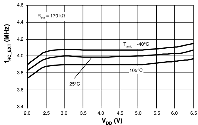
Figure 11-8. External RC Frequency versus V_{DD}
