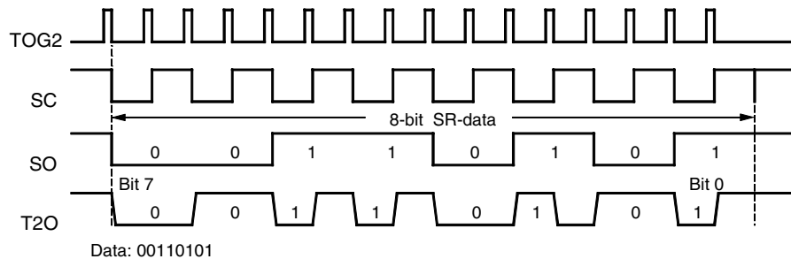
Figure 4-35. Bi-phase Modulation 1
