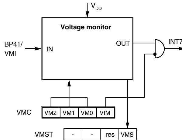
Figure 3-9. Voltage Monitor
