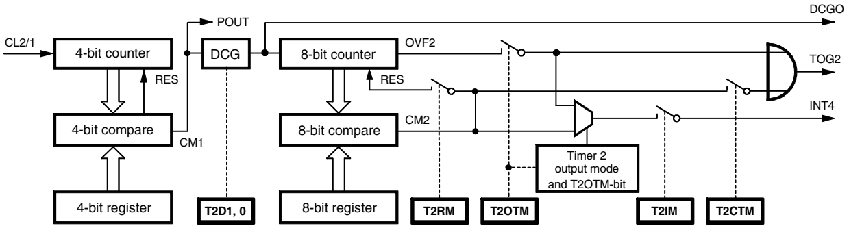
Figure 4-11. 8-bit Compare Counter
