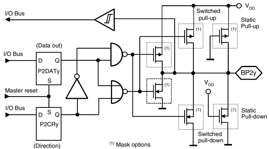
Figure 4-2. Bi-directional Port 2
