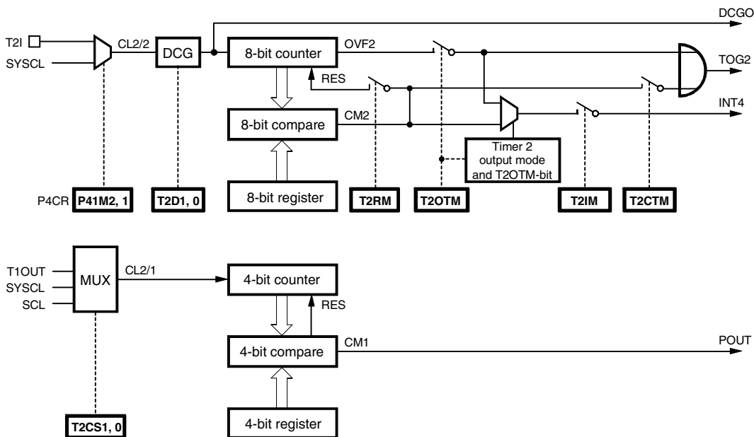
Figure 4-12. 4-/8-bit Compare Counter
