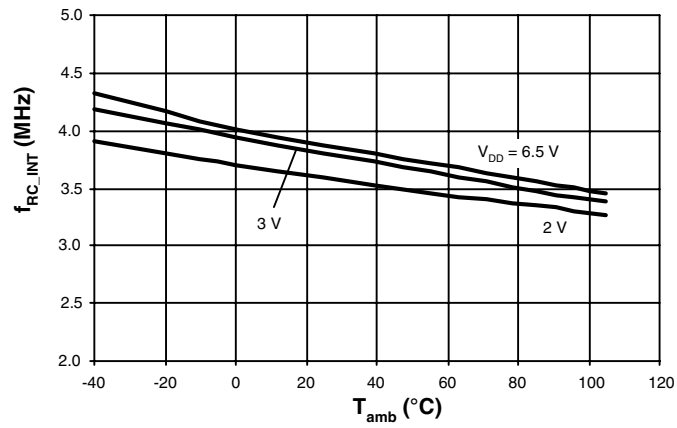
Figure 11-10. Internal RC Frequency versus T_{amb}
