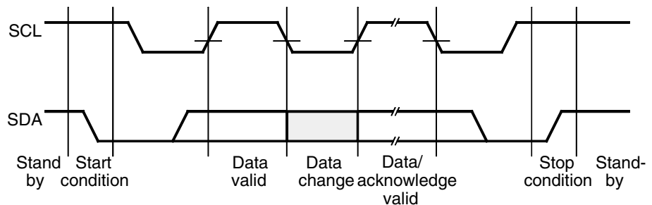
Figure 5-3. I2C Protocol
