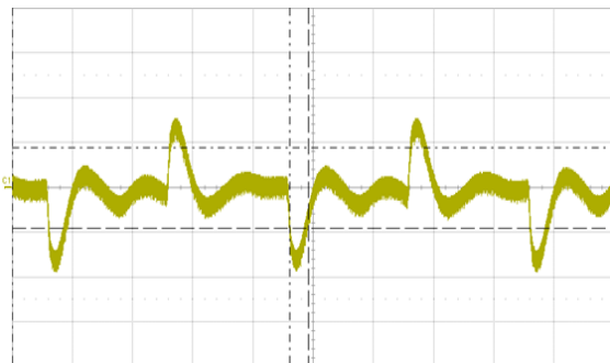
Fig. 11: Output voltage response to load current step-change (1.5 A – 3 A – 1.5 A) at V_{in} = 48\text{ V} . Current slew rate: 0.1 A/ \mu\text{s} . C_o = 270 \mu\text{F} E-cap + 1 \mu\text{F} ceramic + 10 \mu\text{F} tantalum. Time scale: 500 \mu\text{s} /div.
