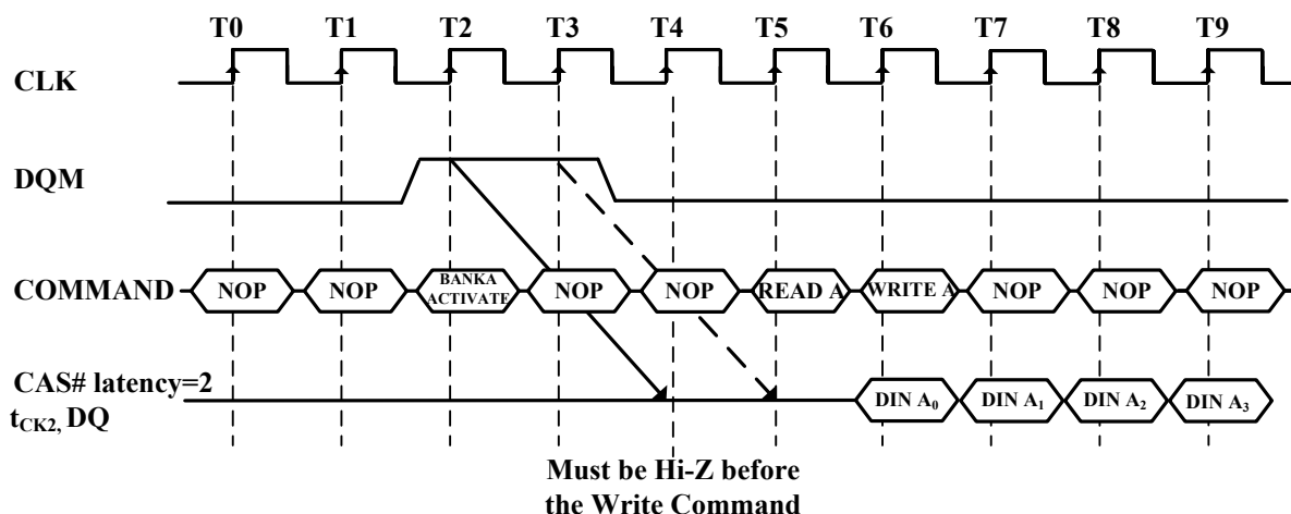
Figure 6. Read to Write Interval (Burst Length ≥ 4, CAS# Latency = 2)
