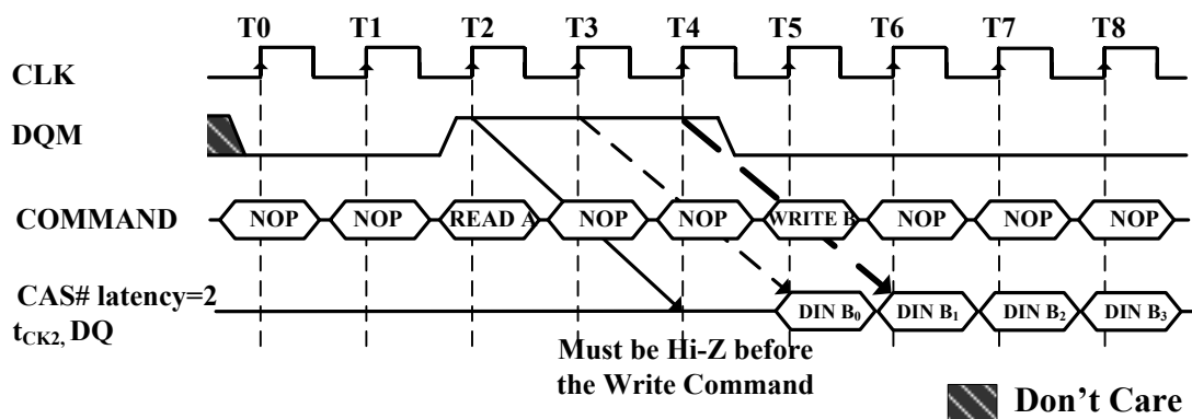
Figure 7. Read to Write Interval (Burst Length ≥ 4, CAS# Latency = 3)
