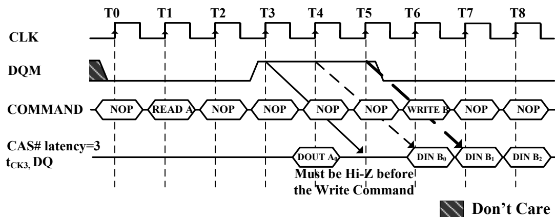
Figure 8. Read to Write Interval (Burst Length ≥ 4, CAS# Latency = 2)
