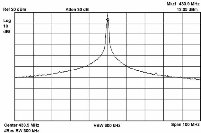
Figure 5-1. Typical RF Spectrum of 40kHz ASK Modulation at P_{out} = 12.5\text{dBm}
