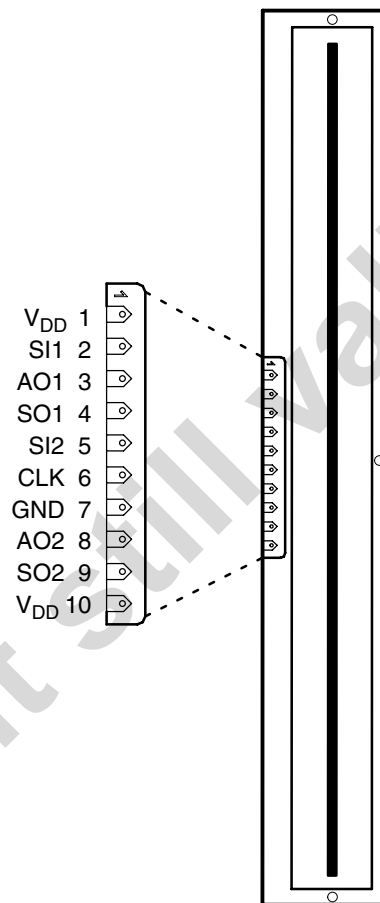
PACKAGE (TOP VIEW)
