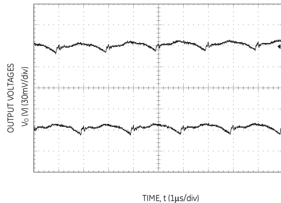
Figure 3. Typical output ripple and noise (C o = 2x0.1μF+2x47μF ceramic, V IN = 12V, I o = I o1,max , I o2,max ).
