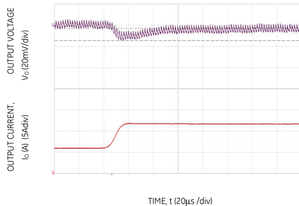
Figure 4. Transient Response to Dynamic Load Change from 50% to 100% on one output at 12Vin, C out =2x47μF+7x330μF, C Tune =12nF, R Tune =300Ω
